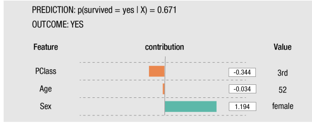
Fig. 3. Example of linear model and the returned features importance.
