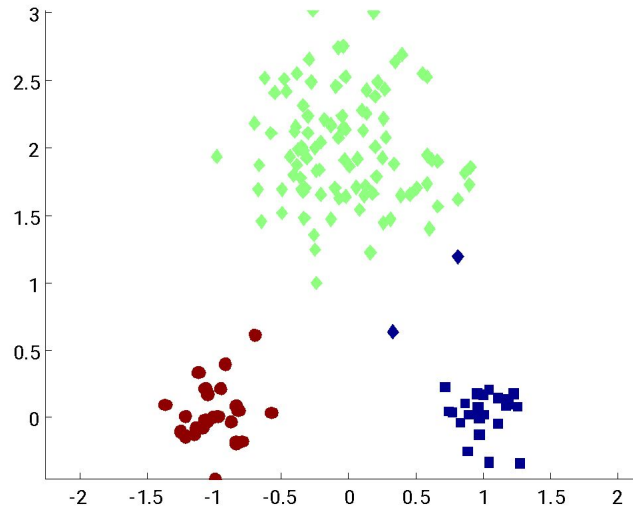
Optimal Clustering
