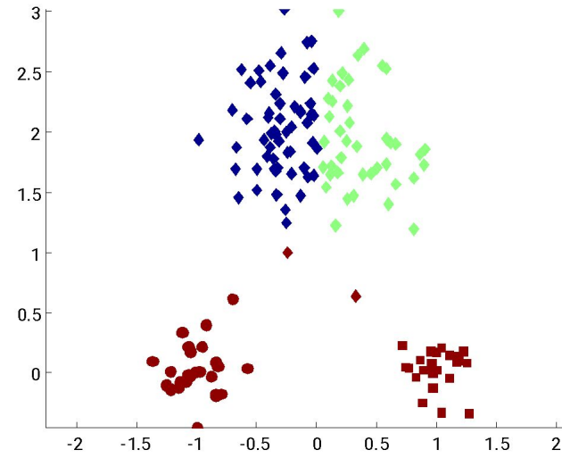
Sub-optimal Clustering
