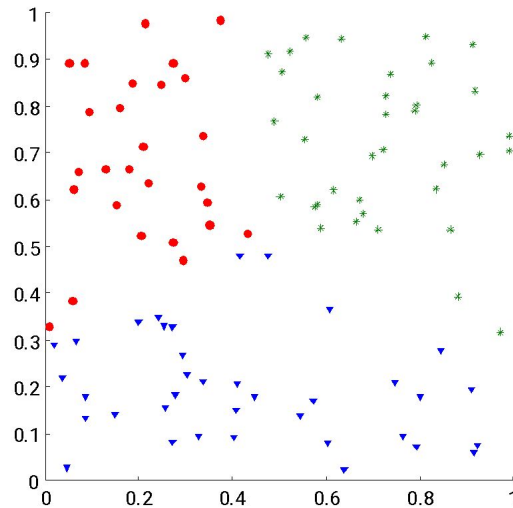
K-means
